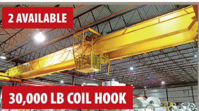
KONE 15-TON X 73' DOUBLE GIRDER BRIDGE CRANE
